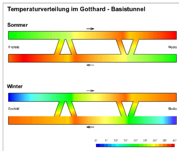
Calculation of climate in the Gotthard base tunnel
