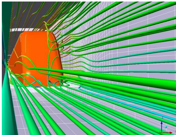
Visualisation of flow through a rail tunnel
