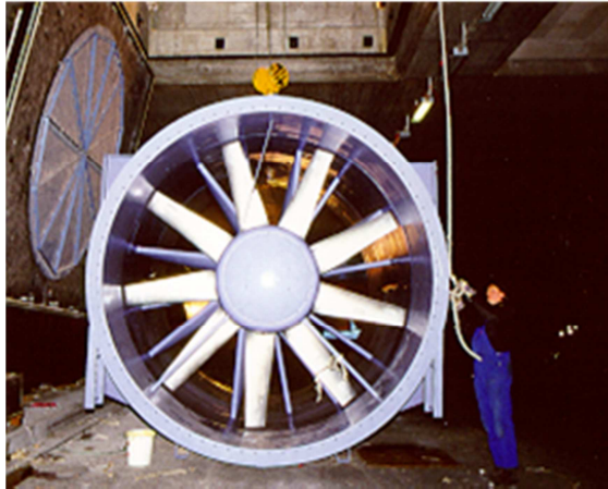
Installation of a fan in a tunnel
