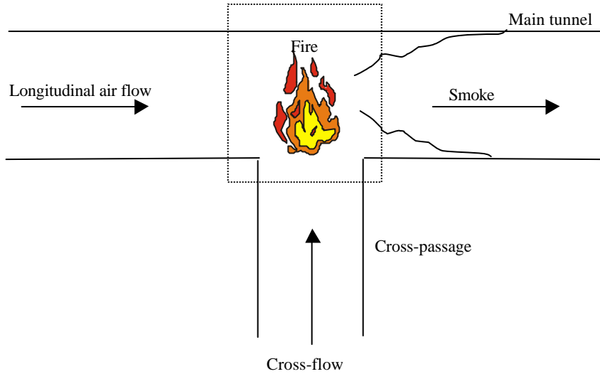
Fig. 3: Control Volume for the Enthalpy Balance in a Tunnel Cross-Passage
