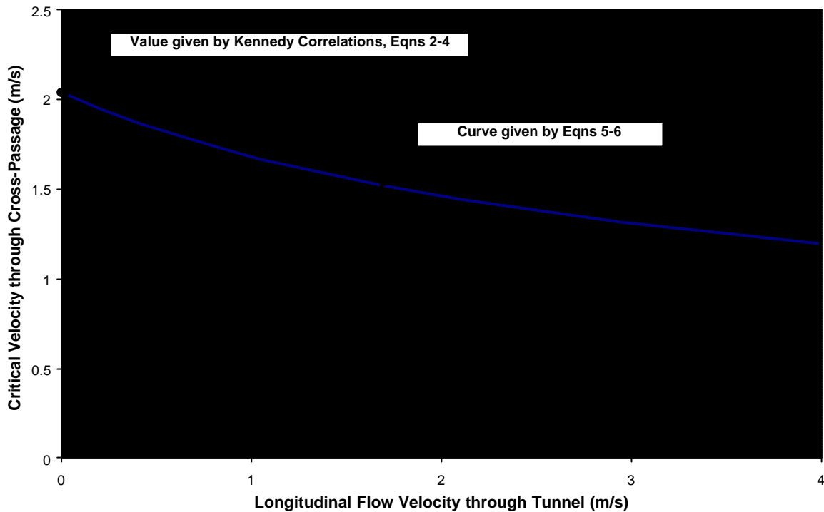
Fig. 4: Variation of Critical Velocity through a Cross-Passage with Longitudinal Tunnel Flow (Example)
