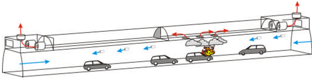
Fig. 6 Ventilation system of the Gotschna tunnel
