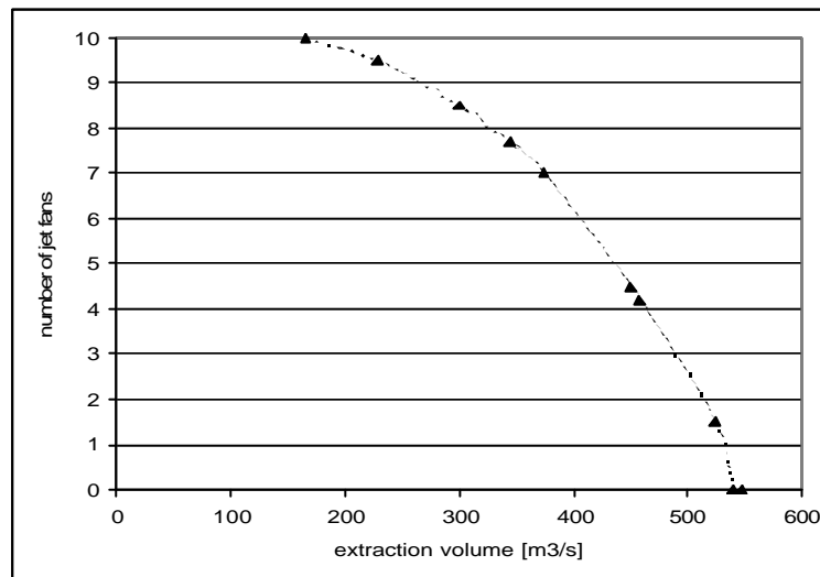
Fig. 5 Smoke extraction volume versus number of jet fans (example)
