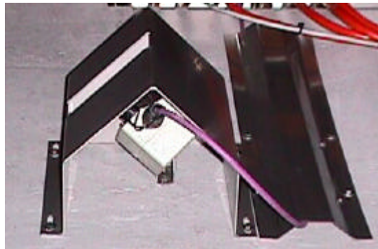
Fig. 8 Ultrasonic anemometer in road tunnel
